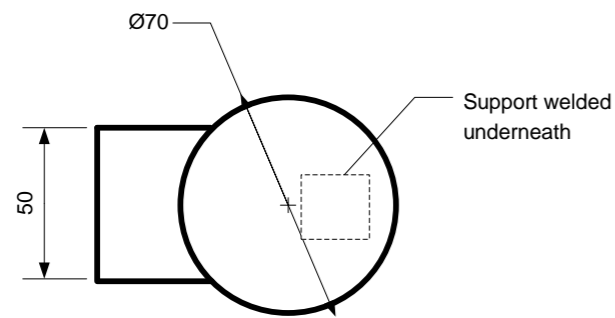
Platform – top view
