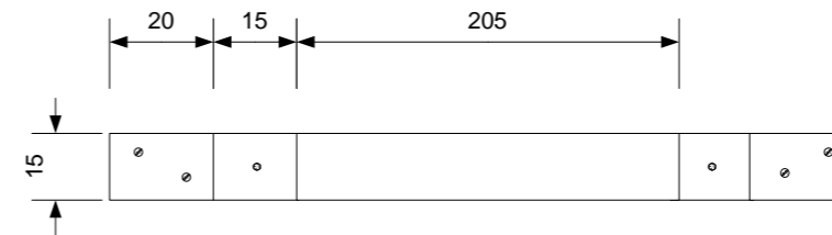
Bottom clamp – flat view
