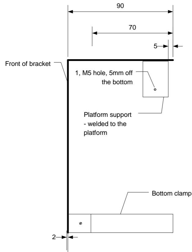
Bracket - side view
