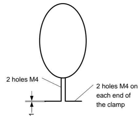
Bottom clamp – top view
